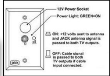
Power Injector
