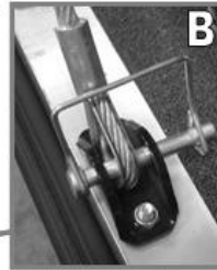
B Safety pin cable hook-up on the cargo ramp door
