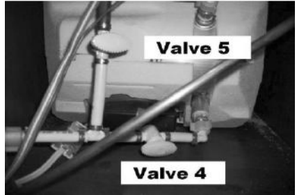
Fig. B - Water Heater Bypass (2 valves)
