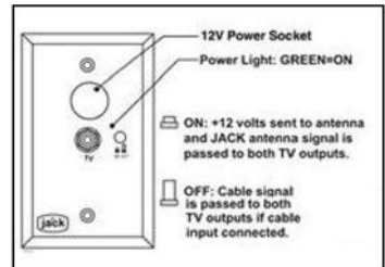
Power Injector
