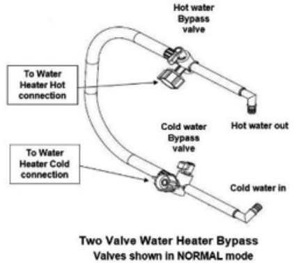
Fig. B - Water Heater Bypass (2 valves)
