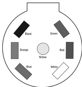
7-way trailer plug - Car end, rear view
