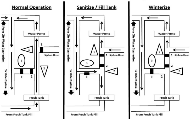
Fig. C - Flow Diagrams
